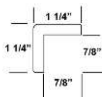
OUTCORN - SHAKER
