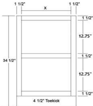
Opening Width Calculation Cabinet Width - 3" = X
