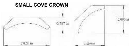
SMALL COVE CROWN
