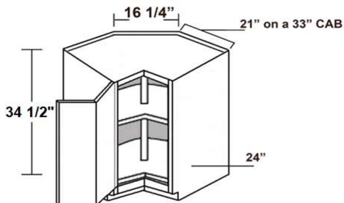
BASE EASY REACH BER33 WITH LAZY SUSAN
