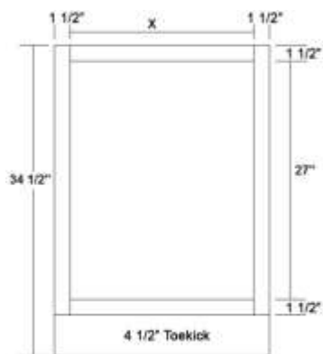
BASE W/ FULL HEIGHT DOOR
