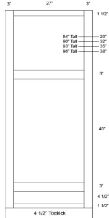
Opening Calculation Cabinet Width 33"
