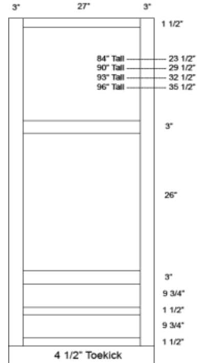
Opening Calculation Cabinet Width 33"
