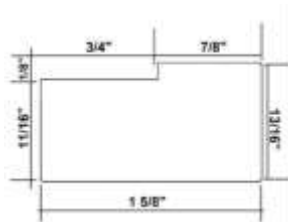
LIGHT RAIL - SHAKER
