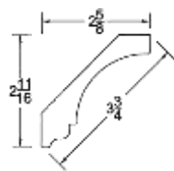
COVE CROWN
