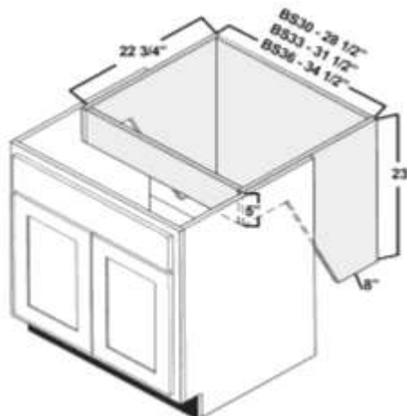
BS-HC30-COMBO-M
