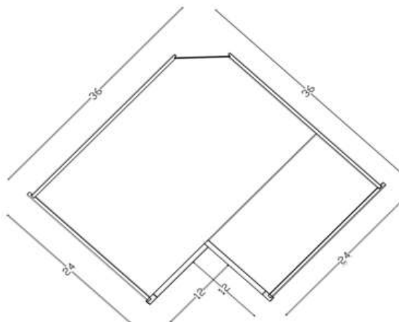
BASE EASY REACH BER36 WITH TWO ADJUSTABLE SHELVES
