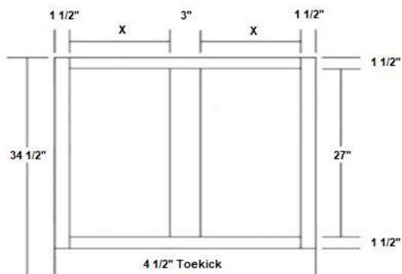
BASE 42", 45" & 48" W/ MULLION & FULL HEIGHT DOOR
