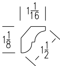
COVE CROWN
