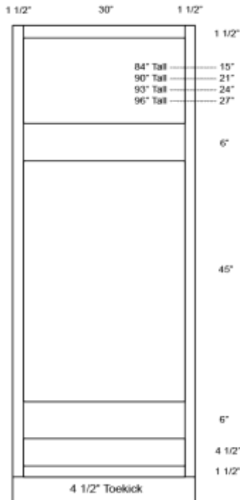
Opening Calculation Cabinet Width 33"
