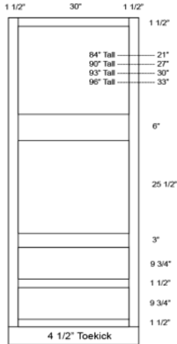
Opening Calculation Cabinet Width 33"
