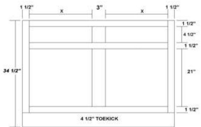
Opening Width Calculation Drawer Opening is Cabinet Width - 6" / 2 = X
