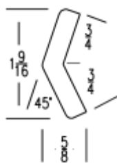
LIGHT RAIL - SHAKER
