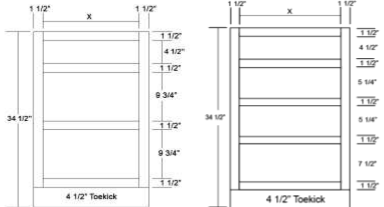
Opening Width Calculation Cabinet Width - 3" = X
