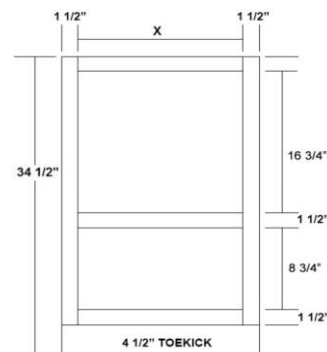
Opening Width Calculation Cabinet Width - 3" = X
