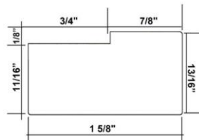
LIGHT RAIL - SHAKER
