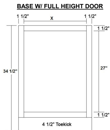
Opening Width Calculation Cabinet Width - 3" = X
