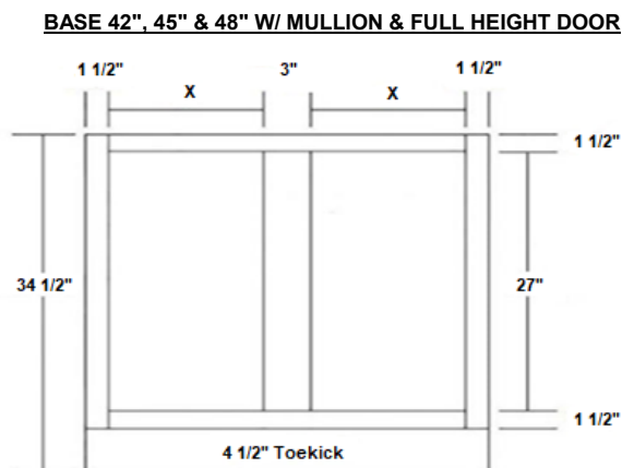
Opening Width Calculation Door Opening is Cabinet Width - 6" / 2 = X
