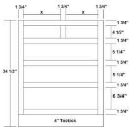
Four Drawer Base with Split Top Drawer
