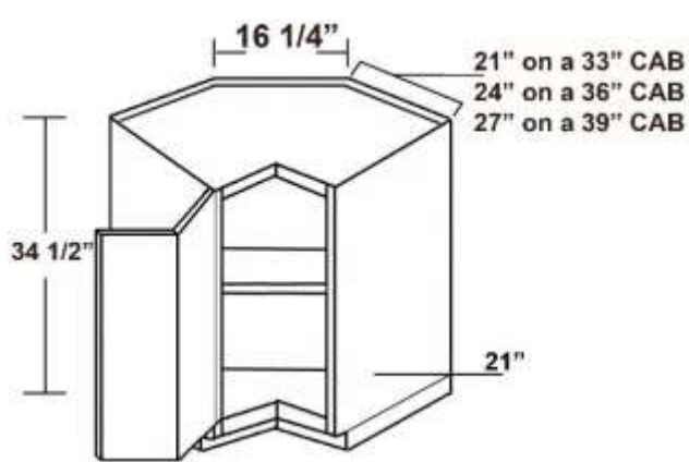
AH Vanity Base Easy Reach
