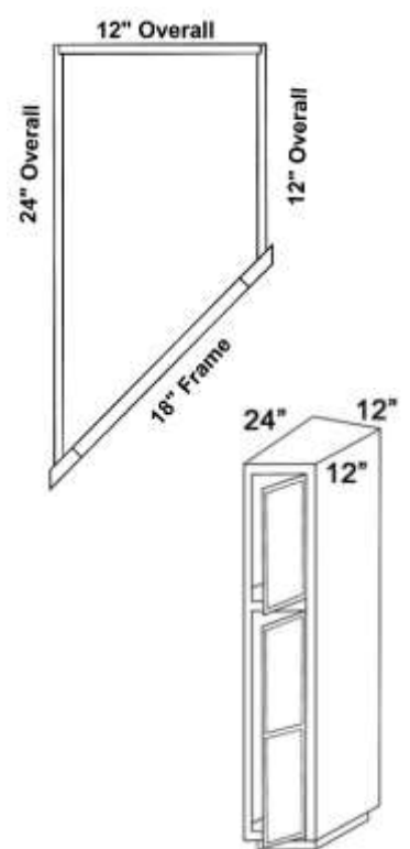
Angled Base Utility End Top View
