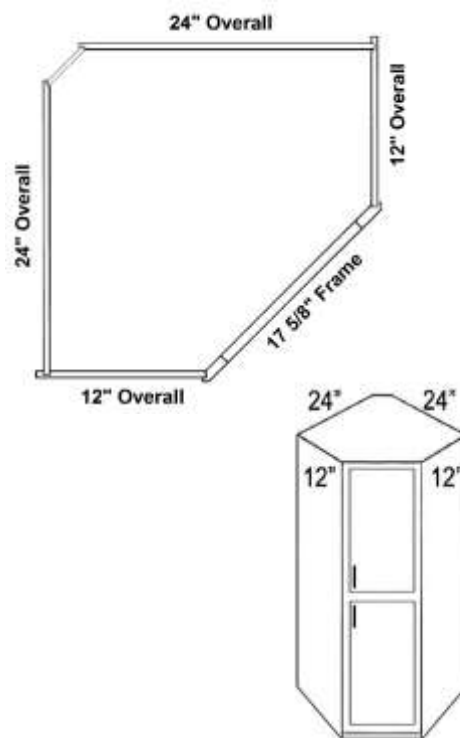
Angled Corner Linen Top View
