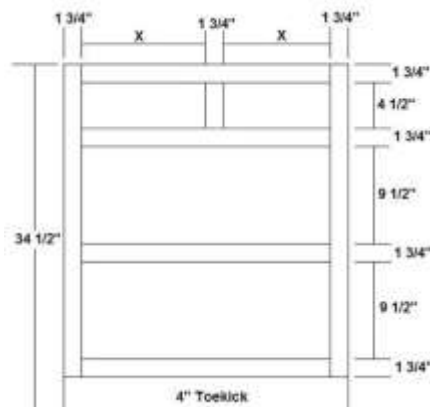
Three Drawer Base with Split Top Drawer
