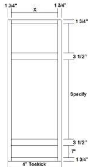
Double Oven Cabinet
