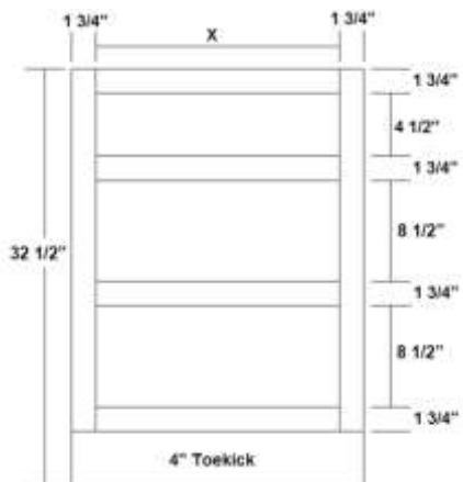
Vanity 3 Drawer Base
