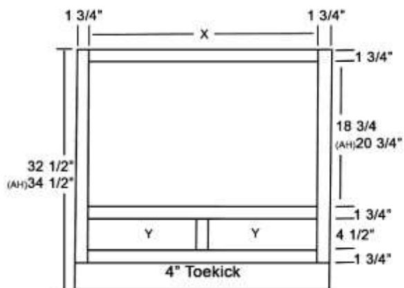
Inverted Sink Base with One Drawer
