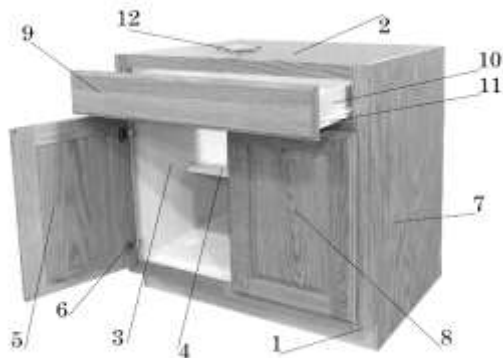
BASE CABINET
