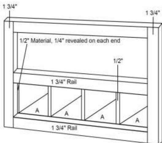
Wall Apothecary 27" thru 30"
