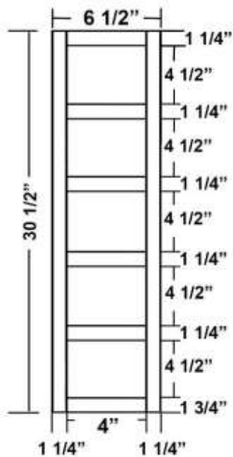
Base Wine W/Face Frame - NTK
