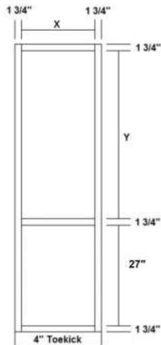
Pantry/Linen Inverted Cabinet 34 1/2" Tall Lower Section
