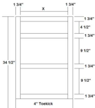
Three Drawer Base
