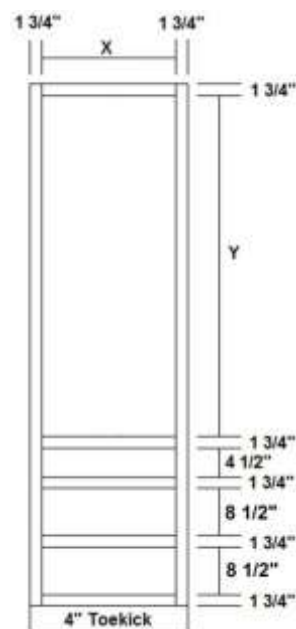
Linen Cabinet W/3 DWRS 32 1/2" Tall Lower Section
