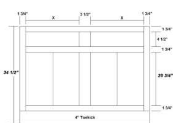
AH Vanity Base with Two Drawers and Four Butt Doors VB48-4B
