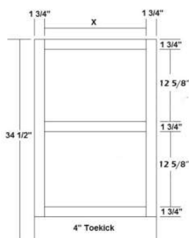
Wine Cradle with Butt Doors or Drawers
