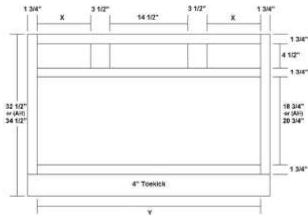
Vanity Base W/Side Drawers 36"- 45" Wide
