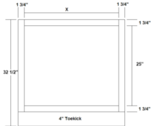
Vanity Base W/Full Height Doors
