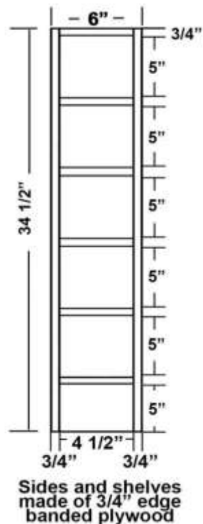
Base Wine Cubbie - FTK
