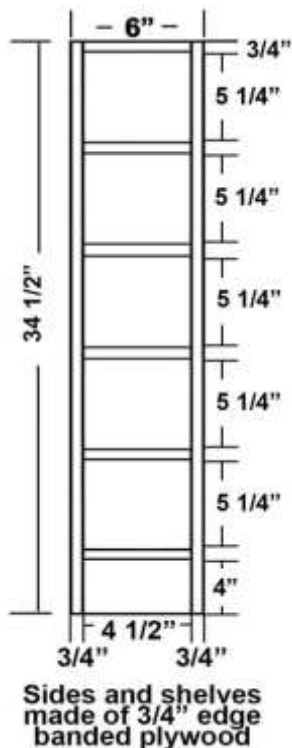
Base Wine Cubbie - RTK
