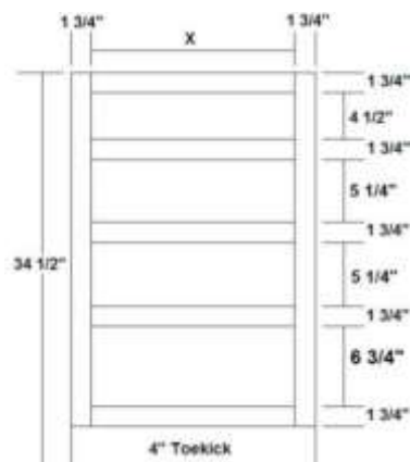
Four Drawer Base
