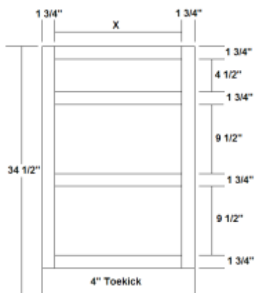
Three Drawer Corner Base W/90 Degree Drawers
