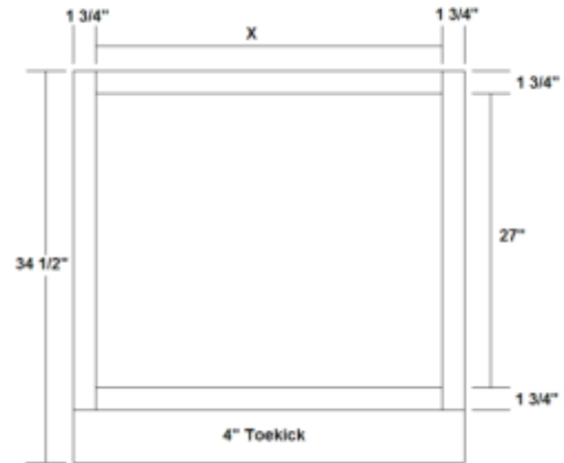
AH Vanity Base W/Full Height Doors
