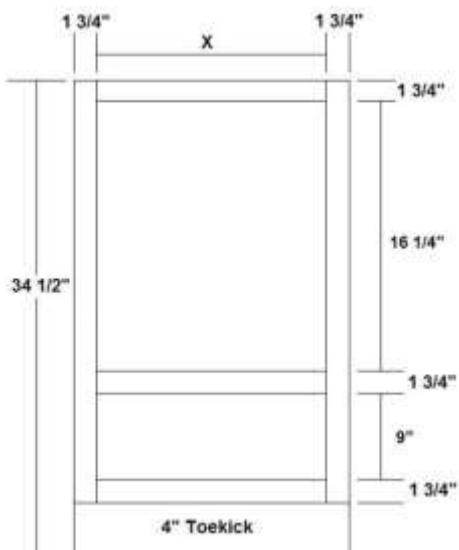
Base Microwave with Drawer
