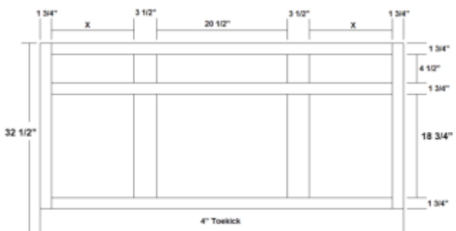
Vanity Base W/Side Drawers 48"- 72" Wide
