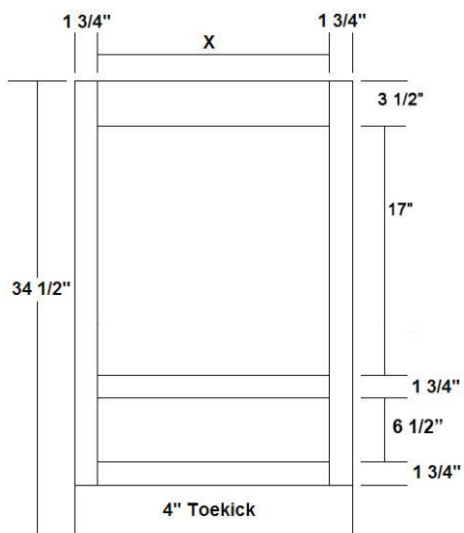
Built in Base Microwave with Drawer
