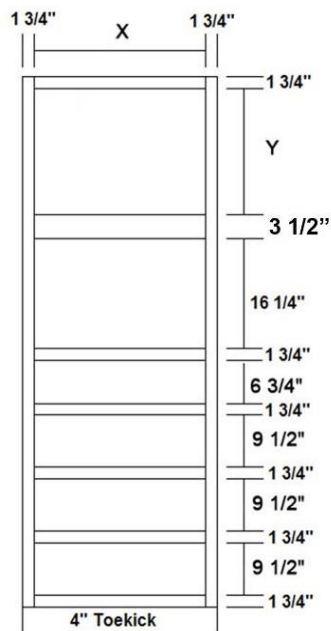
Microwave Oven Cabinet W/4 Drawers
