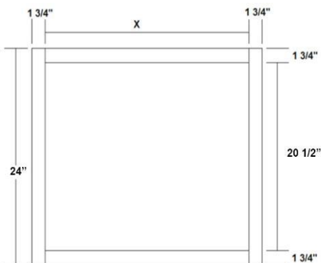
Wall Hung Vanity Sink Base with Full Height Doors
