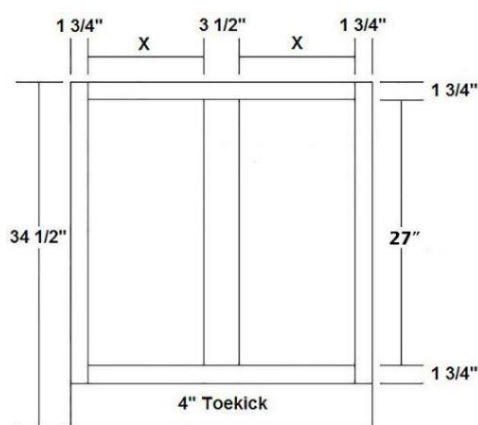
Base with Full Height Door B-48FHD and B48FHD-4B to B60FHD-4B
