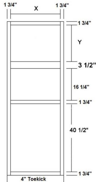
Microwave Oven Cabinet with doors
