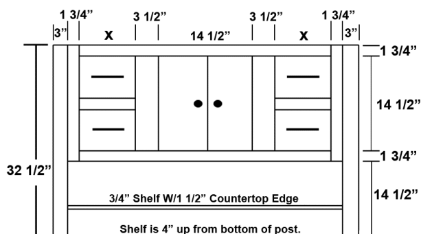
Vanity Furniture Base W/4 Drawers
