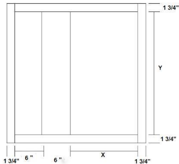
Wall Blind Corner with 1 Door or 2 Butt Doors
