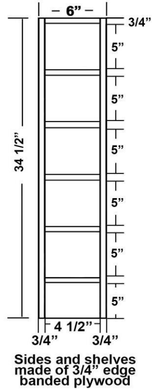
Base Wine Cubbie - FTK
