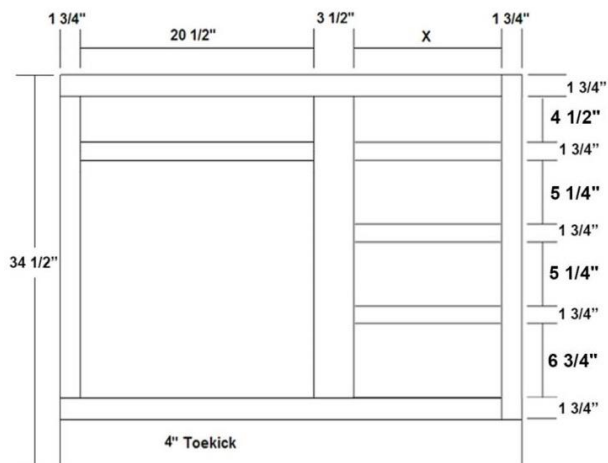
AH Vanity Base W/4 Tub Drawers
