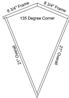
AH Vanity Base Easy Reach
