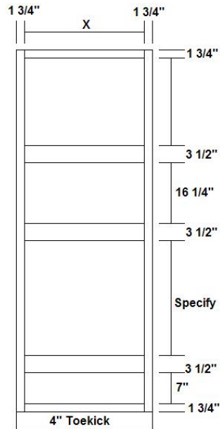
Microwave & Single Oven Cabinet
