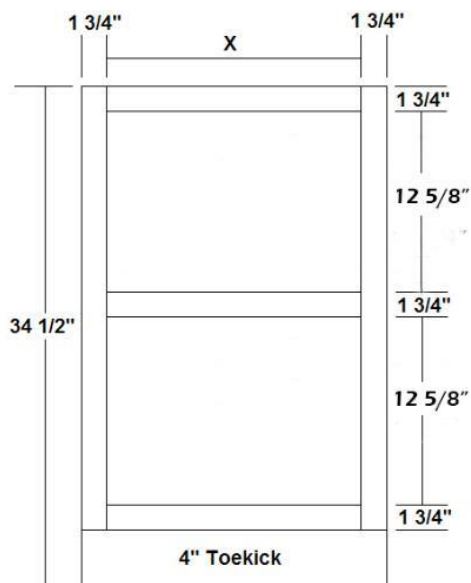
Base Pots and Pans with 2 Drawers
