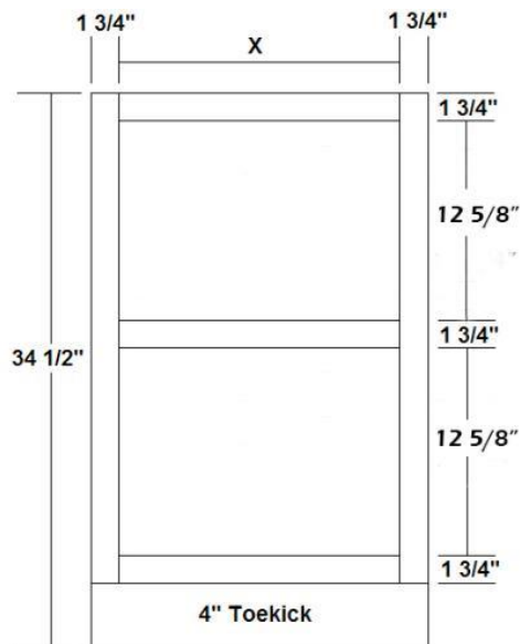
Base Pots and Pans with 1 Drawer and Butt Doors
