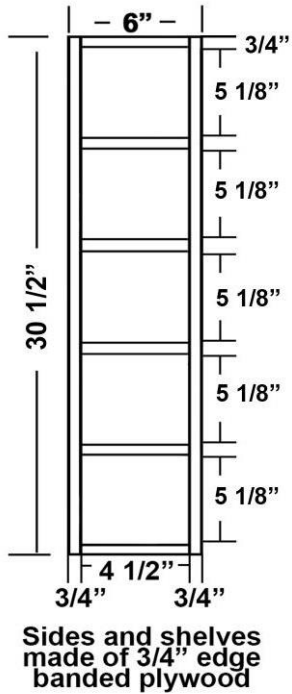
Base Wine Cubbie - NTK
