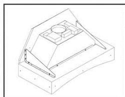
Step 4: Hang the liner/bracket assembly on the mounting plate (make all electrical and ventilation connections at this point)
