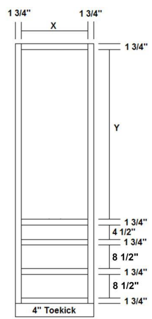
Linen Cabinet W/3 DWRS 32 1/2" Tall Lower Section
