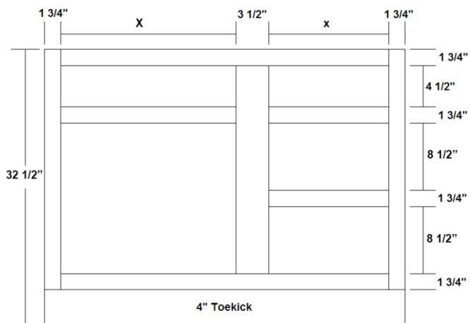
Vanity Base W/3 Tub Drawers
