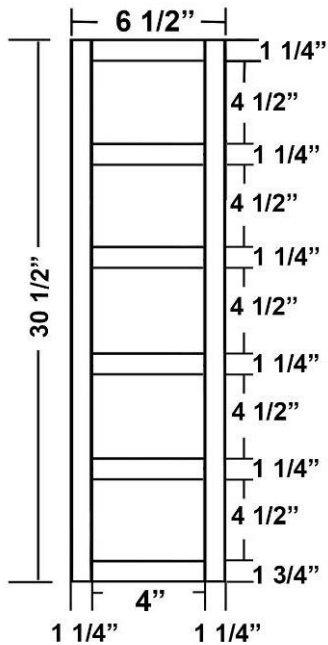
Base Wine W/Face Frame - NTK
