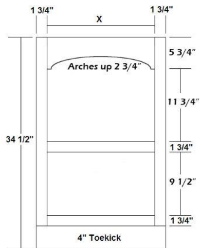
Base Wine Rack W/Valance & Doors
