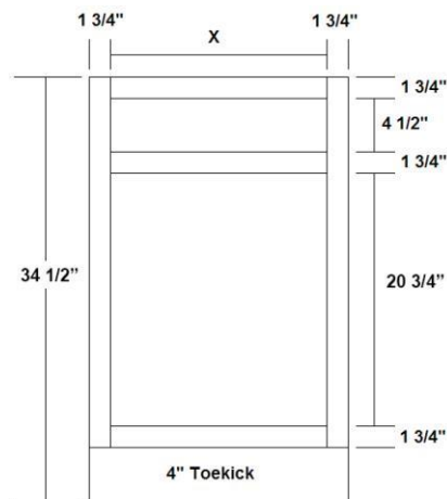
AH Vanity Base 12" to 39" wide
