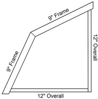
Diagonal Angle 12" Deep - Top View
