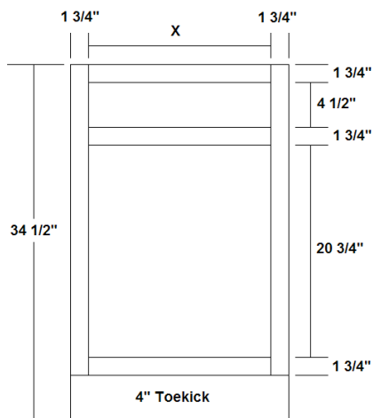
Standard Base with One Drawer B9 thru B39-2B
