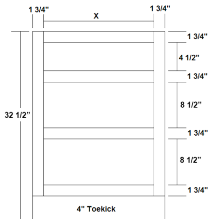
Vanity 3 Drawer Base
