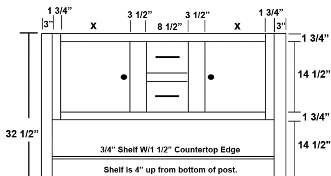
Vanity Furniture Base W/2 Doors & 2 Drawers
