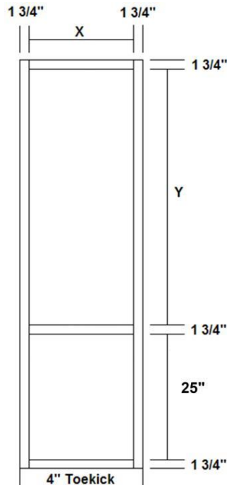
Linen Inverted Cabinet 32 1/2" Tall Lower Section
