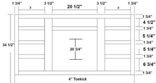
AH Vanity Base W/8 Double Drawers - 48" thru 72" Wide
