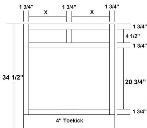
Standard Base with Two Drawers & Two Butt Doors B42-2B & B45-2B
