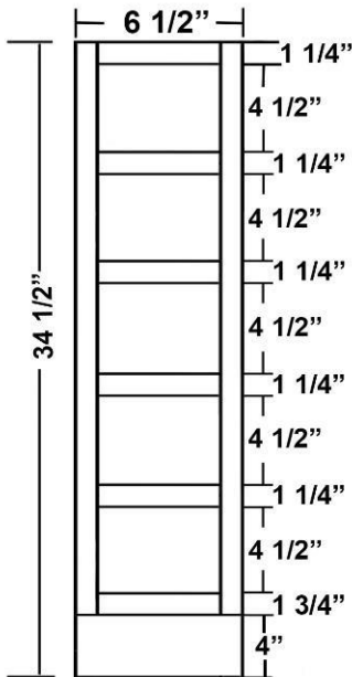
Base Wine W/Face Frame - RTK
