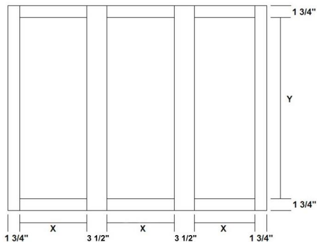
Standard Wall with 3 Doors
