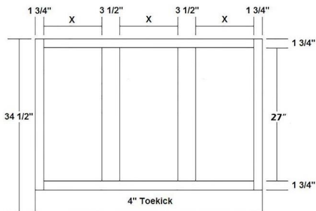
Base with Full Height Door B51FHD to B60FHD
