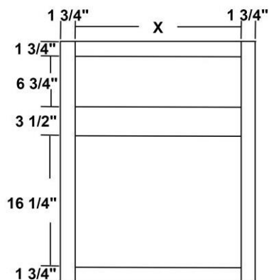
Built in Microwave Cabinet 30" Tall
