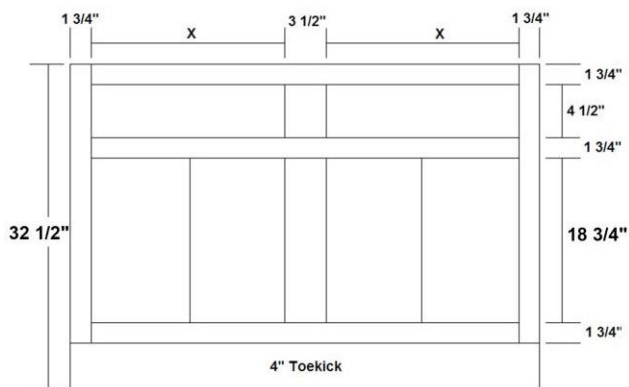
Vanity Base with Two Drawers and Four Butt Doors VB48-4B
