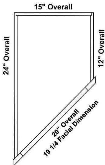
Base Transition Top View BA15U24U12
