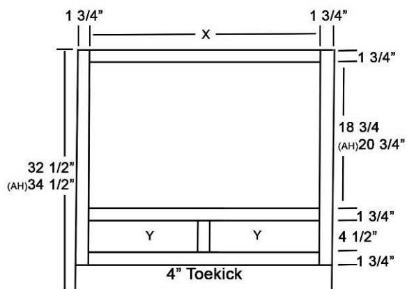
Inverted Sink Base with One Drawer
