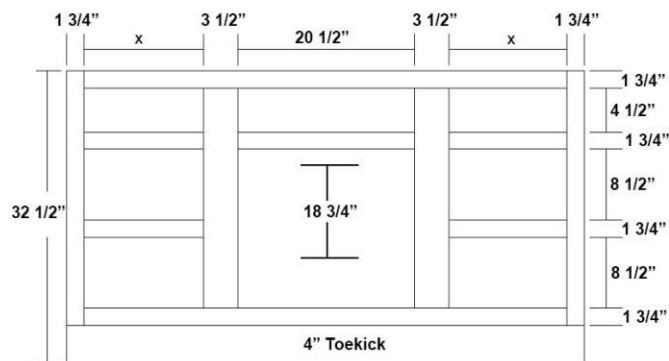
Vanity Base W/6 Double Drawers - 48" thru 72" Wide
