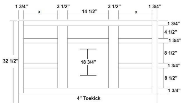
Vanity Base W/6 Double Drawers - 42" or 45" wide
