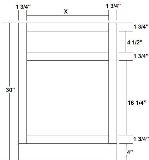
Office Base W/Drawer - Recessed Toe
