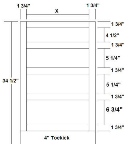
AH Vanity 4 Drawer Base
