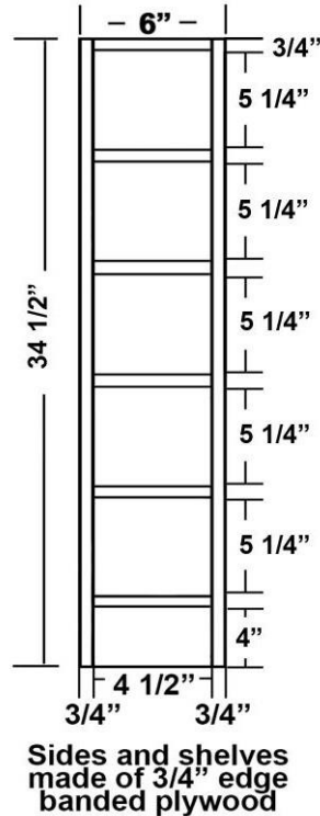
Base Wine Cubbie - RTK
