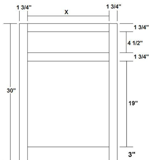
Office Base W/Drawer - Flush Toe
