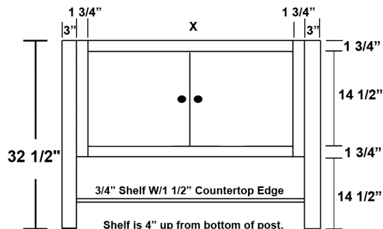
Vanity Furniture Base W/2 Doors
