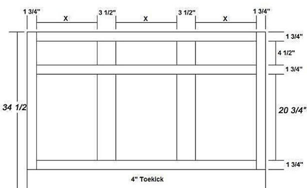
Standard Base with 3 Drawers and 3 Doors
