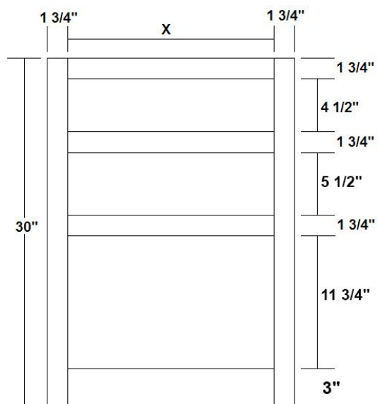
File Base W/Two STD DWRS & 1 File DWR - Flush Toe
