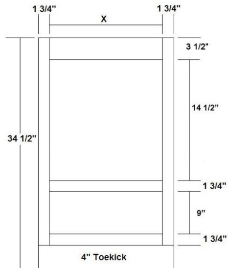
Base W/Built in Microwave Drawer and Lower Drawer
