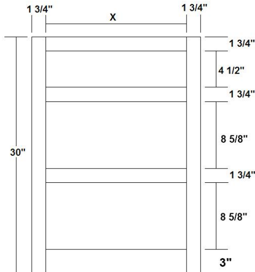
Three Drawer Base With Flush Toe
