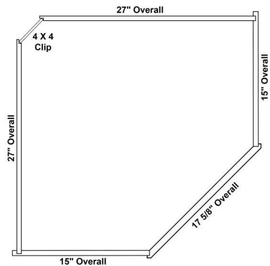
27W - 15" Deep Diagonal Wall Cabinets - Top View
