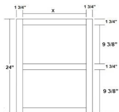
Wall Hung Vanity Base with Two Drawers
