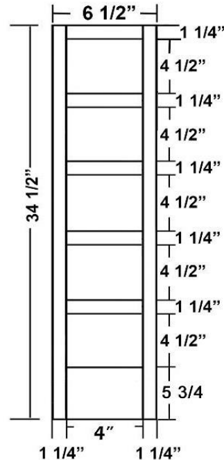
Base Wine W/ Face Frame - FTK
