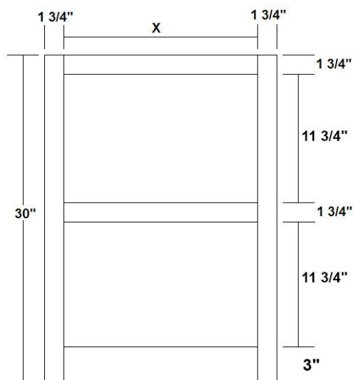
File Base With 2 File DWRS - Flush Toe
