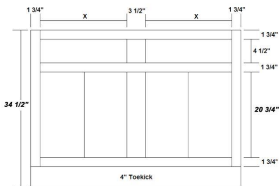
AH Vanity Base with Two Drawers and Four Butt Doors VB48-4B
