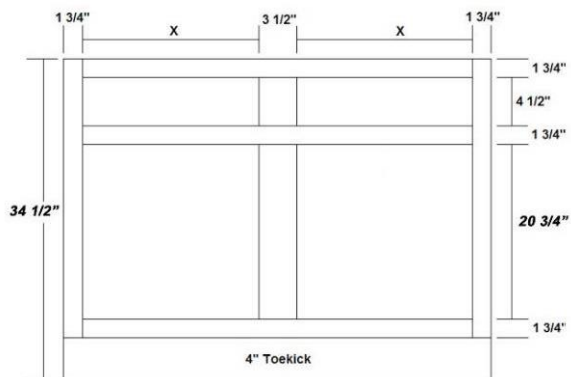
Standard Base with 2 Drawers and 4 Butt Doors B48-4B and B-48 with 2 Doors
