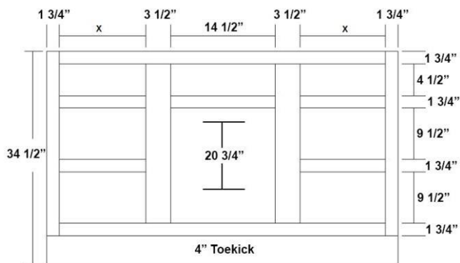
AH Vanity Base W/6 Double Drawers - 42" or 45" Wide
