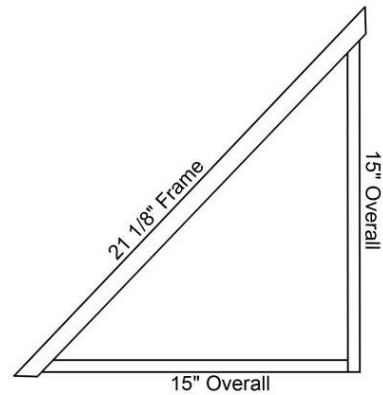
27W - 15" Deep Diagonal Wall Cabinets - Top View
