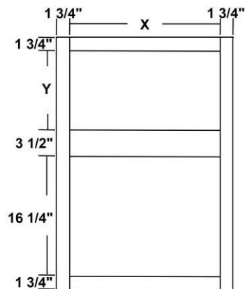
Built in Microwave Cabinet 36" Thru 48" Tall
