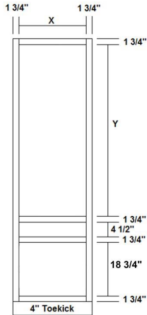
Linen Cabinet W/1 DWR 32 1/2" Tall Lower Section
