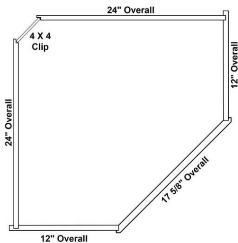
24W - 12" Deep Diagonal Wall Cabinets - Top View
