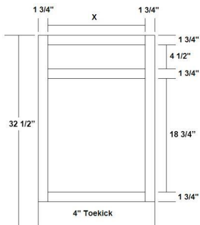
Vanity Base 12" to 39" wide
