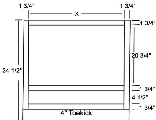
Inverted Sink Base with One Drawer
