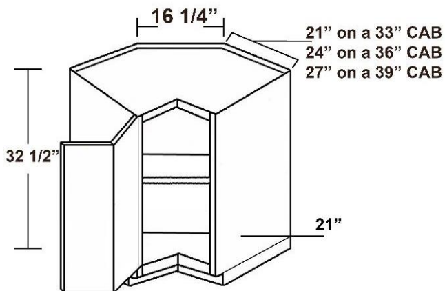
Vanity Base Easy Reach
