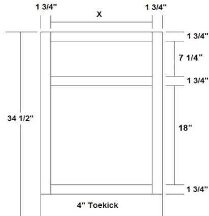
Base with Paper Towel Drawer
