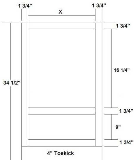
Base Microwave with Drawer
