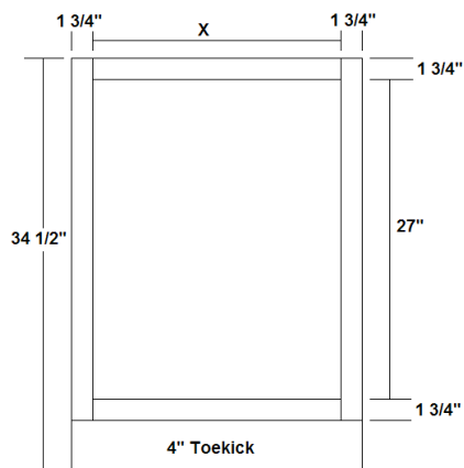
Base with Full Height Door B9FHD to B45FHD-2B
