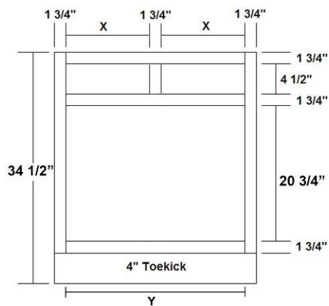
AH Vanity Base 42B" & 45B"
