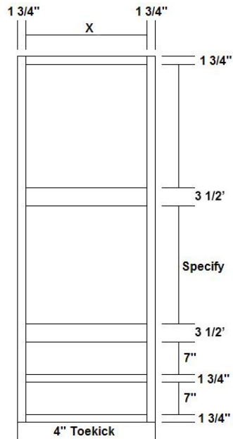
Single Oven Cabinet
