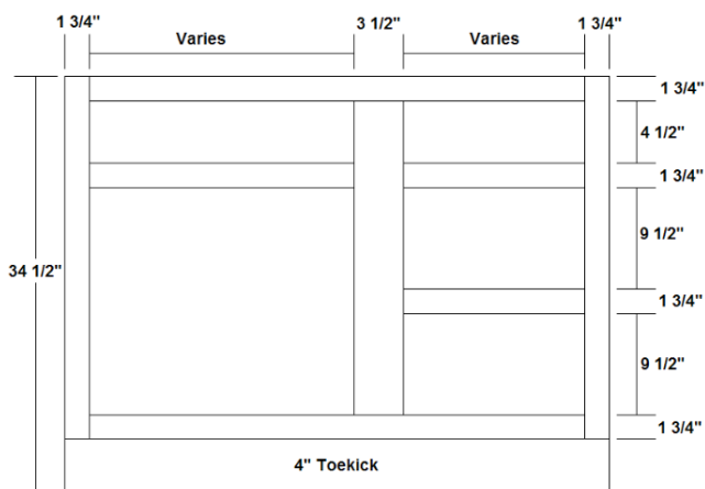
AH Vanity Base W/3 Tub Drawers
