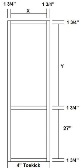
Pantry/Linen Inverted Cabinet 34 1/2" Tall Lower Section
