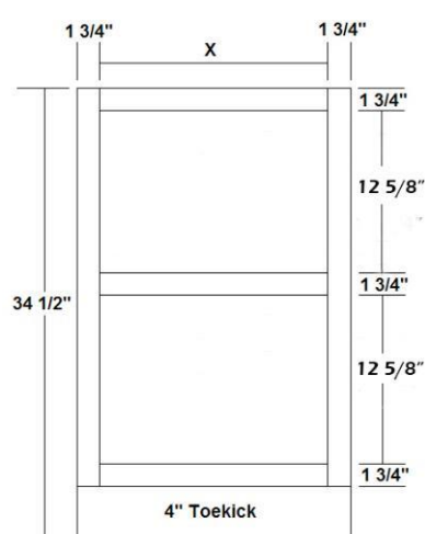
Wine Cradle with Butt Doors or Drawers
