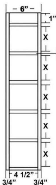
Vertical Wall Wine Cubbie FACE FRAME HAS EDGE BANDING MADE OF 3/4" MATERIAL
