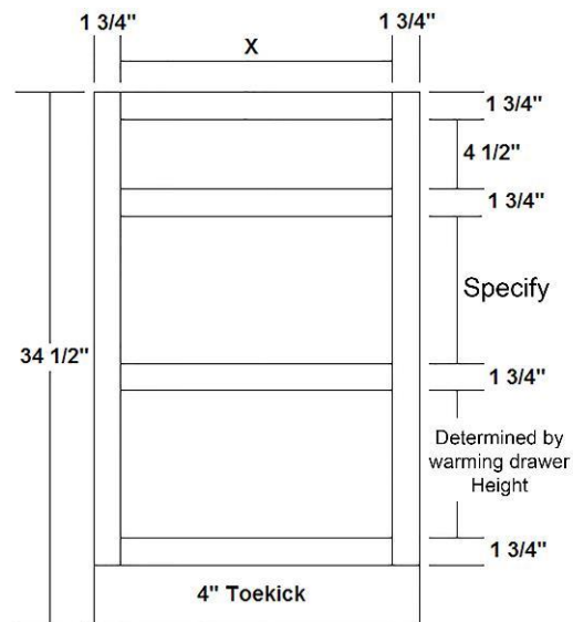
Base with Warming DWR and Two Working DWRS
