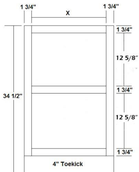
Base Pots and Pans with 2 Drawers and 1 Rollout
