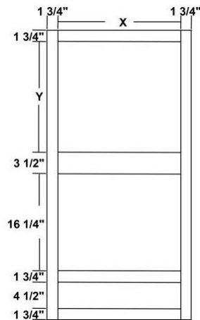
Wall Microwave & One Drawer W/One or Two Butt Doors
