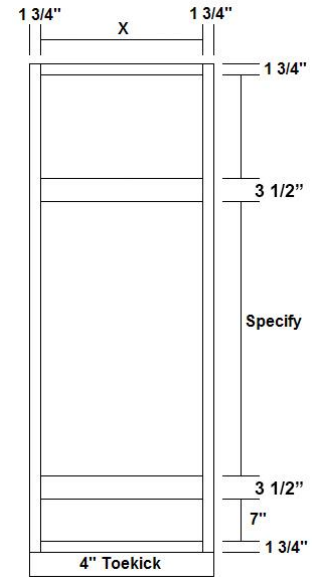
Double Oven Cabinet
