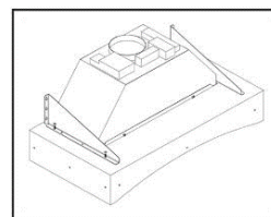
Step 3: Fasten metal mounting brackets to liner
