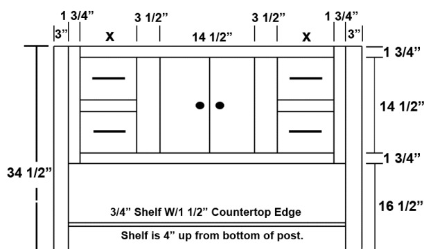
AH Vanity Furniture Base W/4 Drawers
