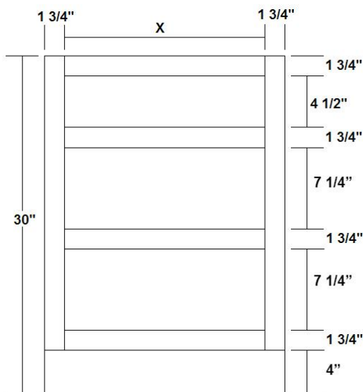
Three Drawer Base With Recessed Toe
