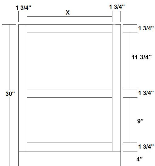
File Base W/1 STD DWR & 1 File DWR - Recessed Toe
