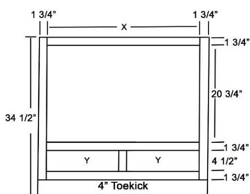
Inverted Sink Base with Two Drawers
