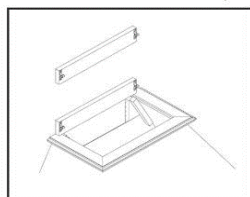
Step 7: If using a chimney (sold separately) mount blocks to wall
