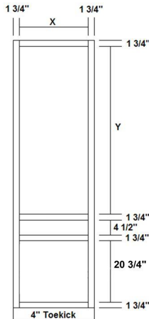
Pantry/Linen Cabinet W/1 DWR 34 1/2" Tall Lower Section
