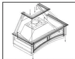
Step 5: Slip the wood range hood on top of the mounting plate
