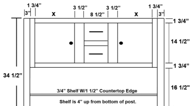
AH Vanity Furniture Base W/2 Doors & 2 Drawers
