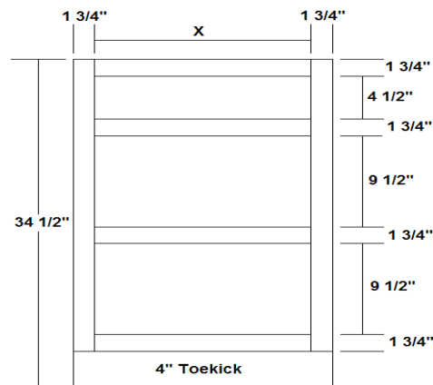
AH Vanity 3 Drawer Base
