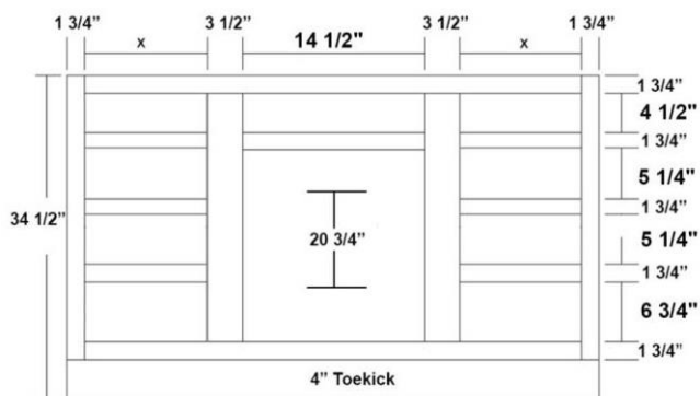
AH Vanity Base W/8 Double Drawers - 42" or 45" Wide
