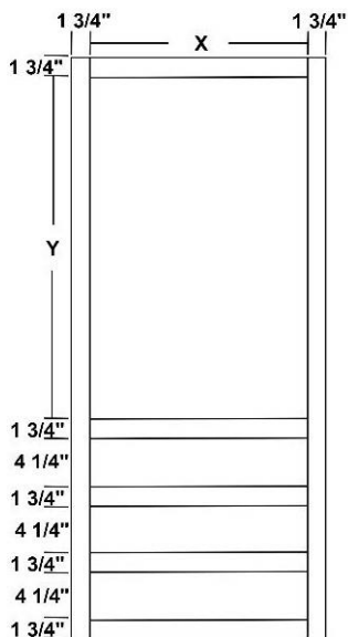
Standard Wall with Three Drawers
