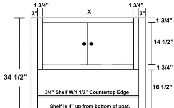
AH Vanity Furniture Base W/2 Doors
