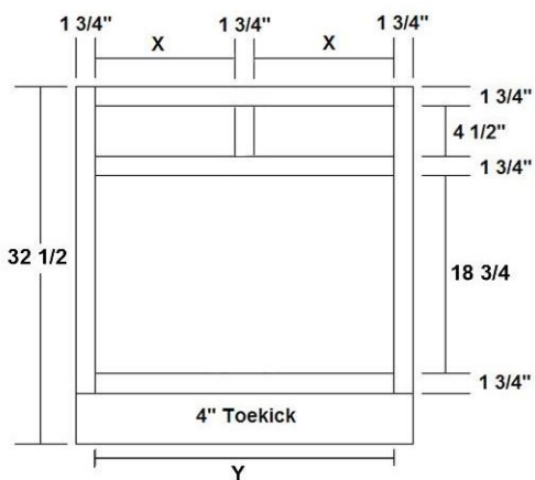
Vanity Base 42B" & 45B"
