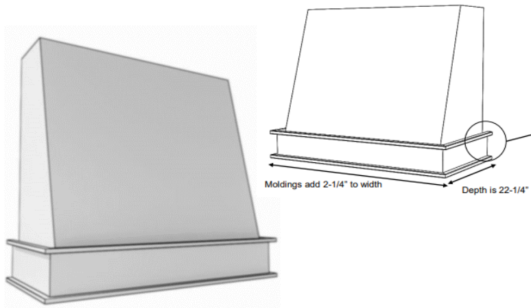
MOLDINGS ADD 2 1/4" TO THE WIDTH 6" BASE / DEPTH IS 22 1/4"
