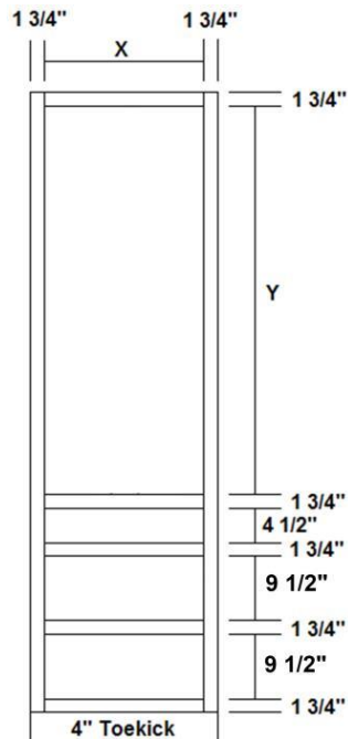
Pantry/Linen Cabinet W/3 DWRS 34 1/2" Tall Lower Section
