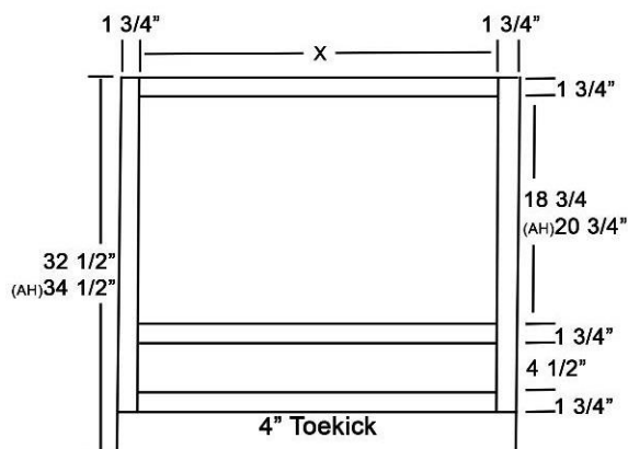
Inverted Sink Base with Two Drawers
