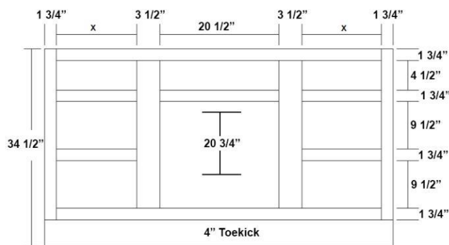
AH Vanity Base W/6 Double Drawers - 48" thru 72" Wide
