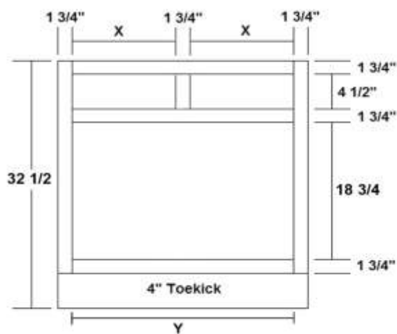
VANITY BASE 42" THRU 48" WIDE
