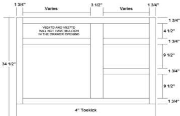
AH VANITY BASE WITH TUB DRAWERS
