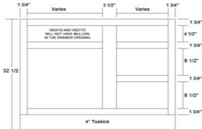
VANITY BASE WITH TUB DRAWERS
