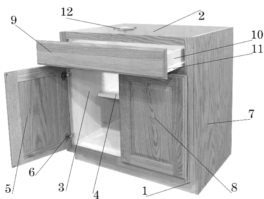
BASE CABINET
