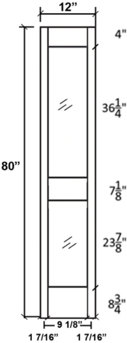
Profile:7799
