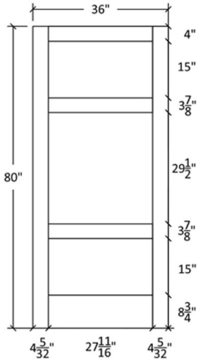
Profile:5426
