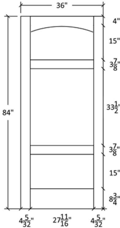
Profile:7797
