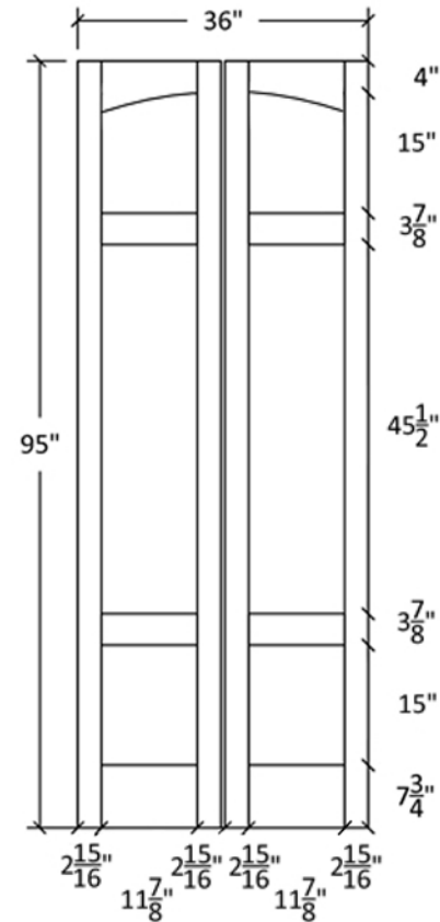
Profile:6715
