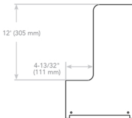
PIPE CLEARANCE DIMENSIONS (For both units)
